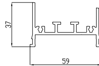
Hand Rail Part 1 Available 6m long, can be joined SCALE 1:1
