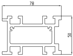
Base Rail Available 6m long, can be joined SCALE 1:1
