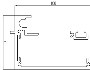
Access Gutter Available 6m long, can be joined SCALE 1:1
