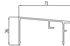
Hand Rail Part 2 Available 6m long, can be joined SCALE 1:1
