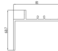
Base Rail Cover 1 Available 6m long, can not be joined SCALE 1:1
