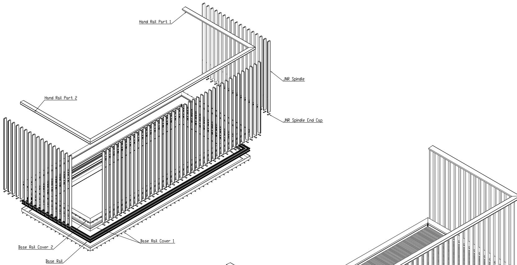
EXPLODED VIEW
