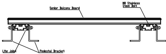
DETAIL A
