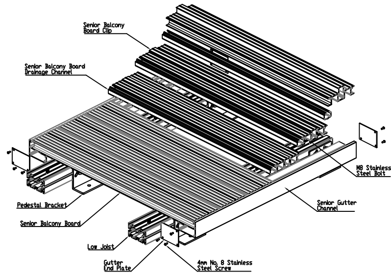
ISOMETRIC VIEW
