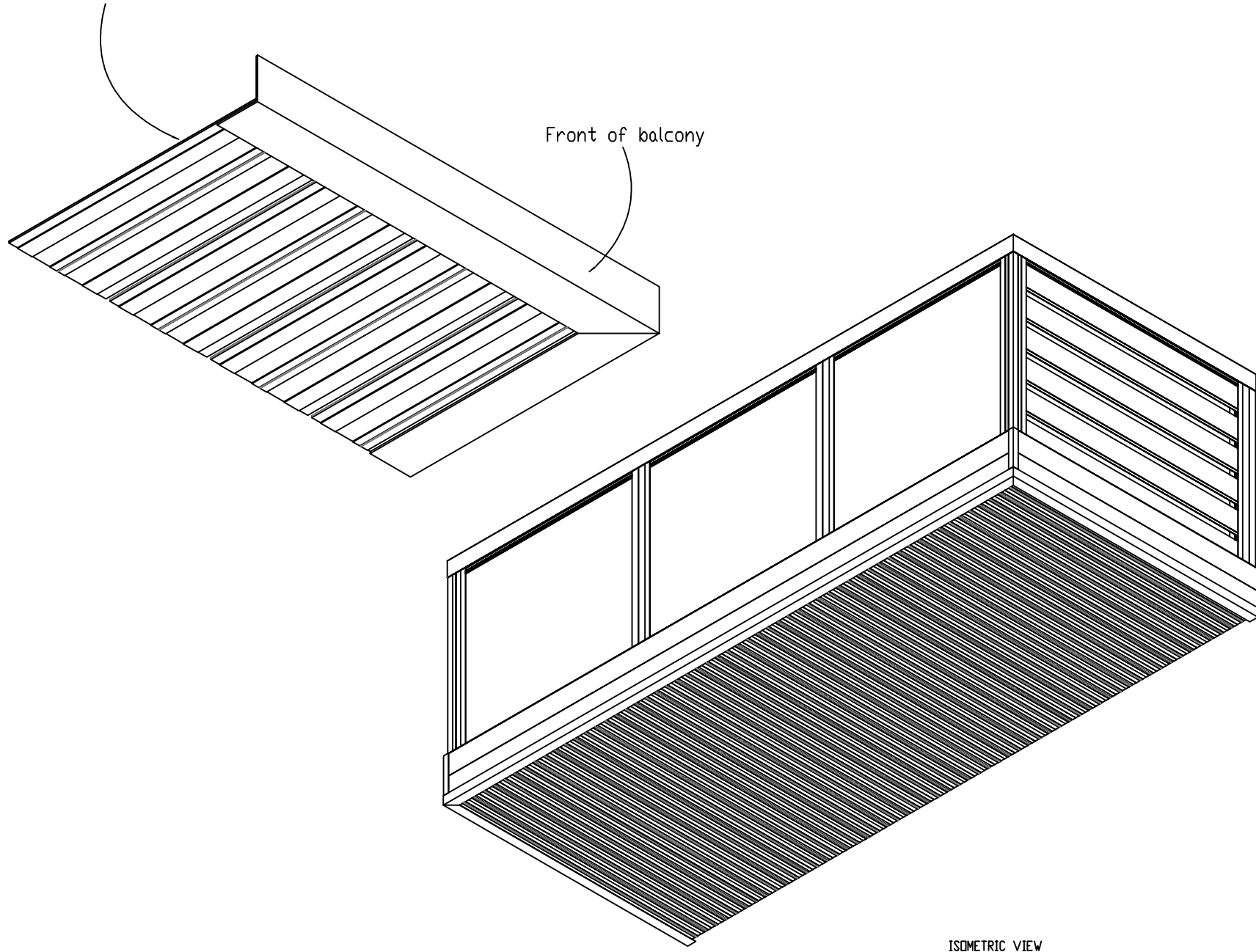
ISOMETRIC VIEW
