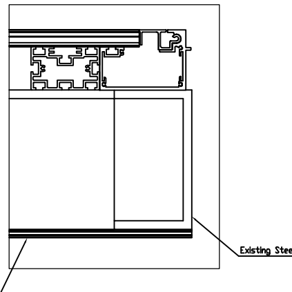
DETAIL O
