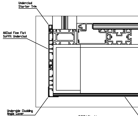
DETAIL N
