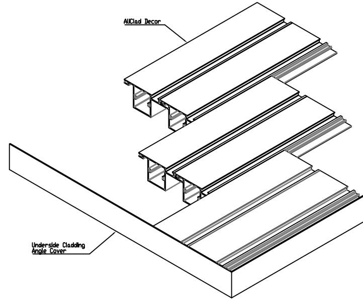
Corner Detail
