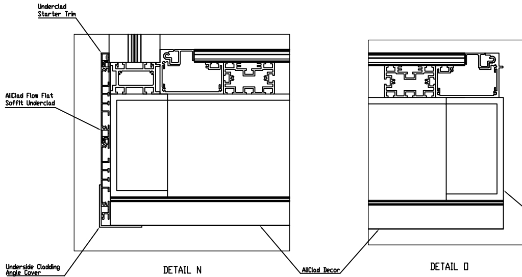
DETAIL N
