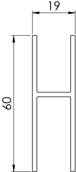
Bottom Rail
