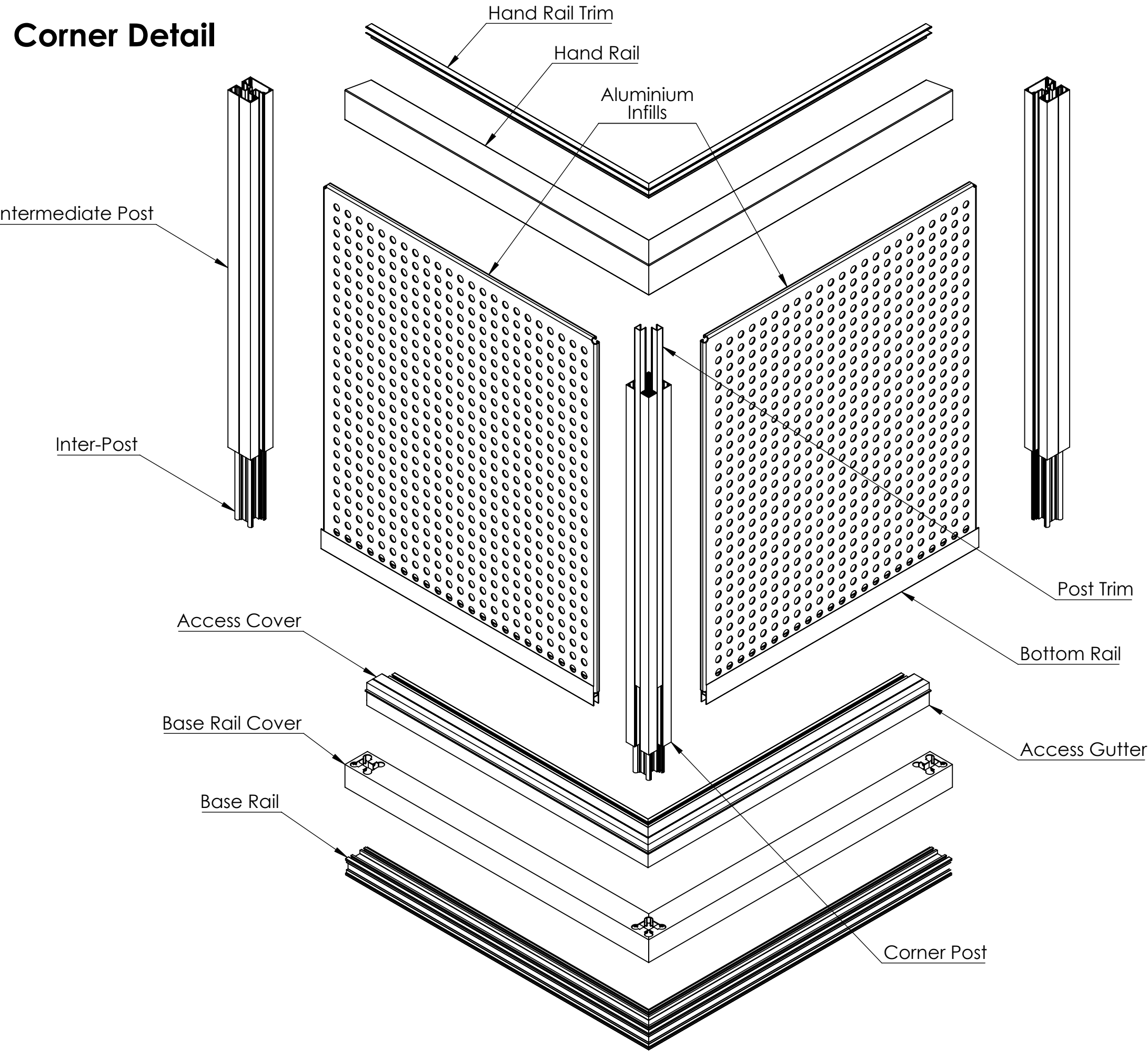
Exploded View
