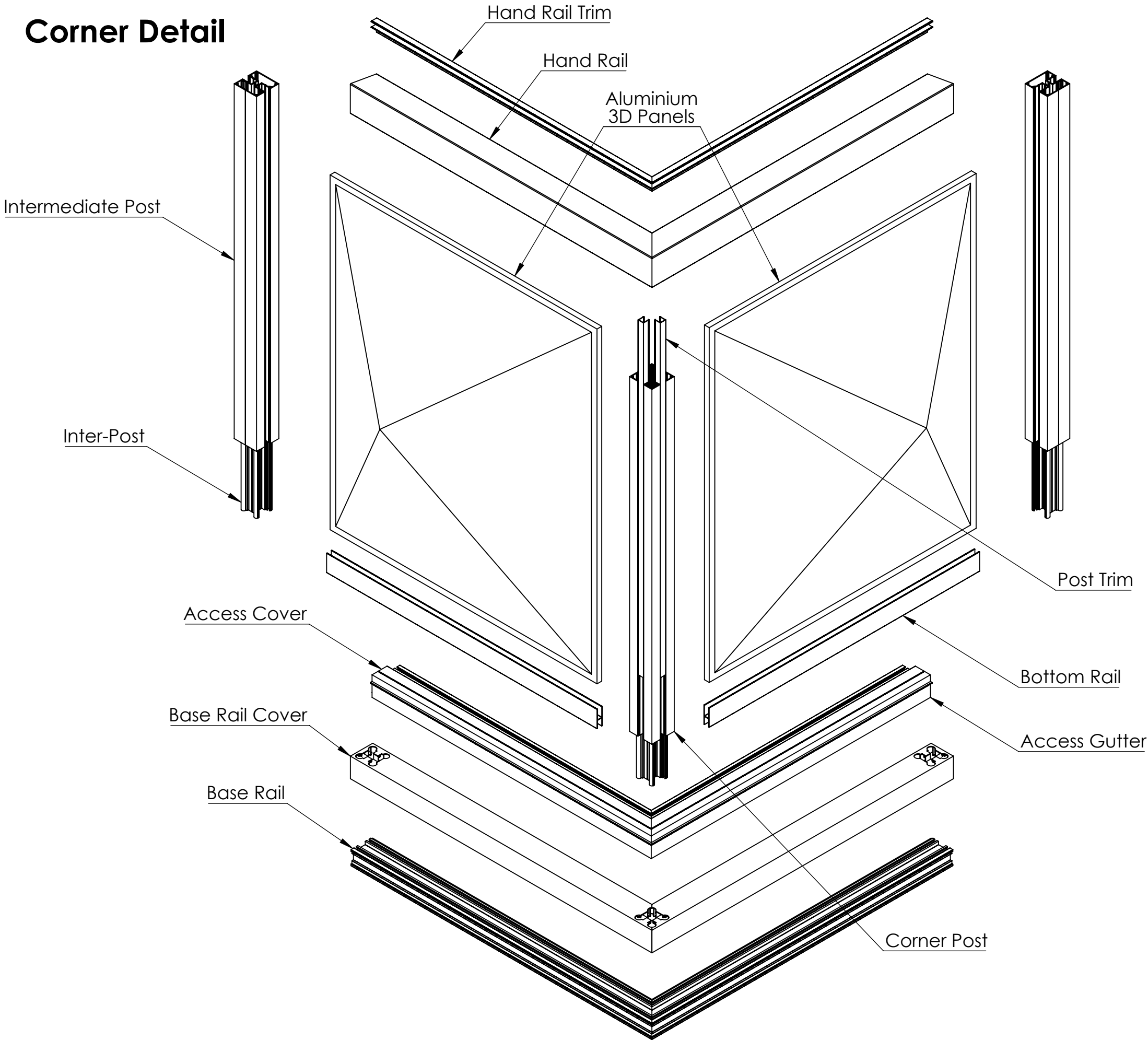
Exploded View
