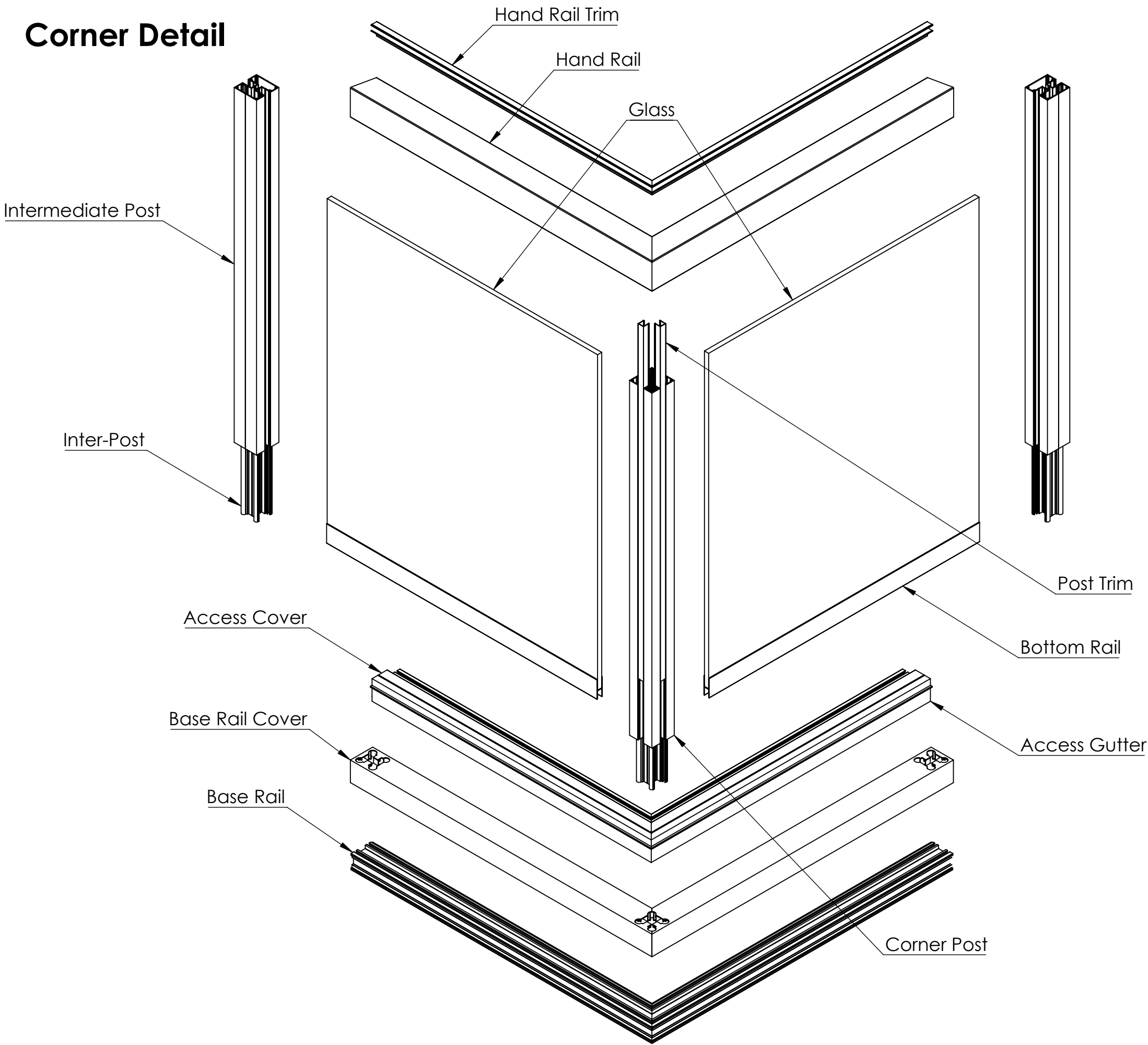
Exploded View
