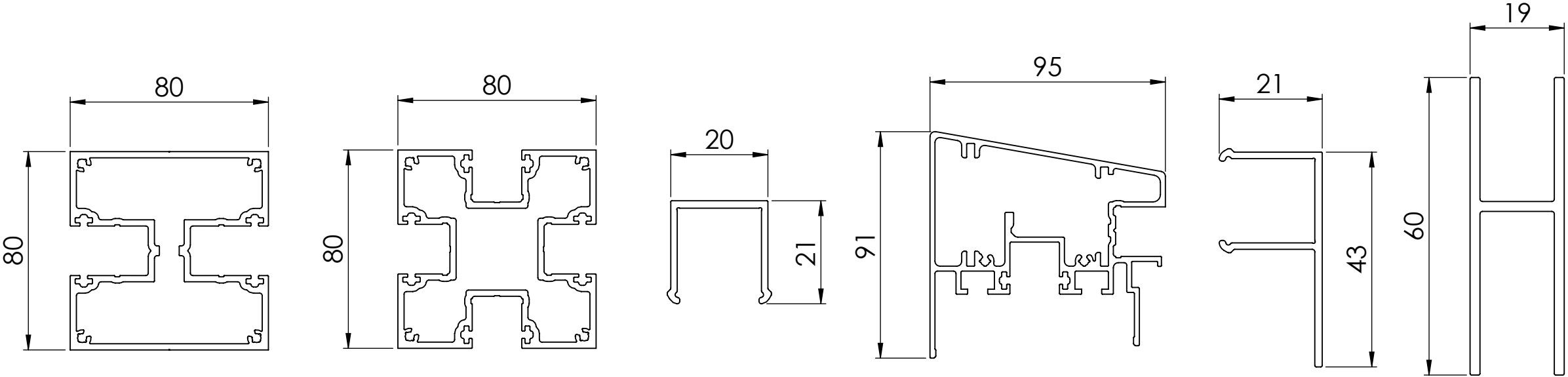
Intermediate Post
