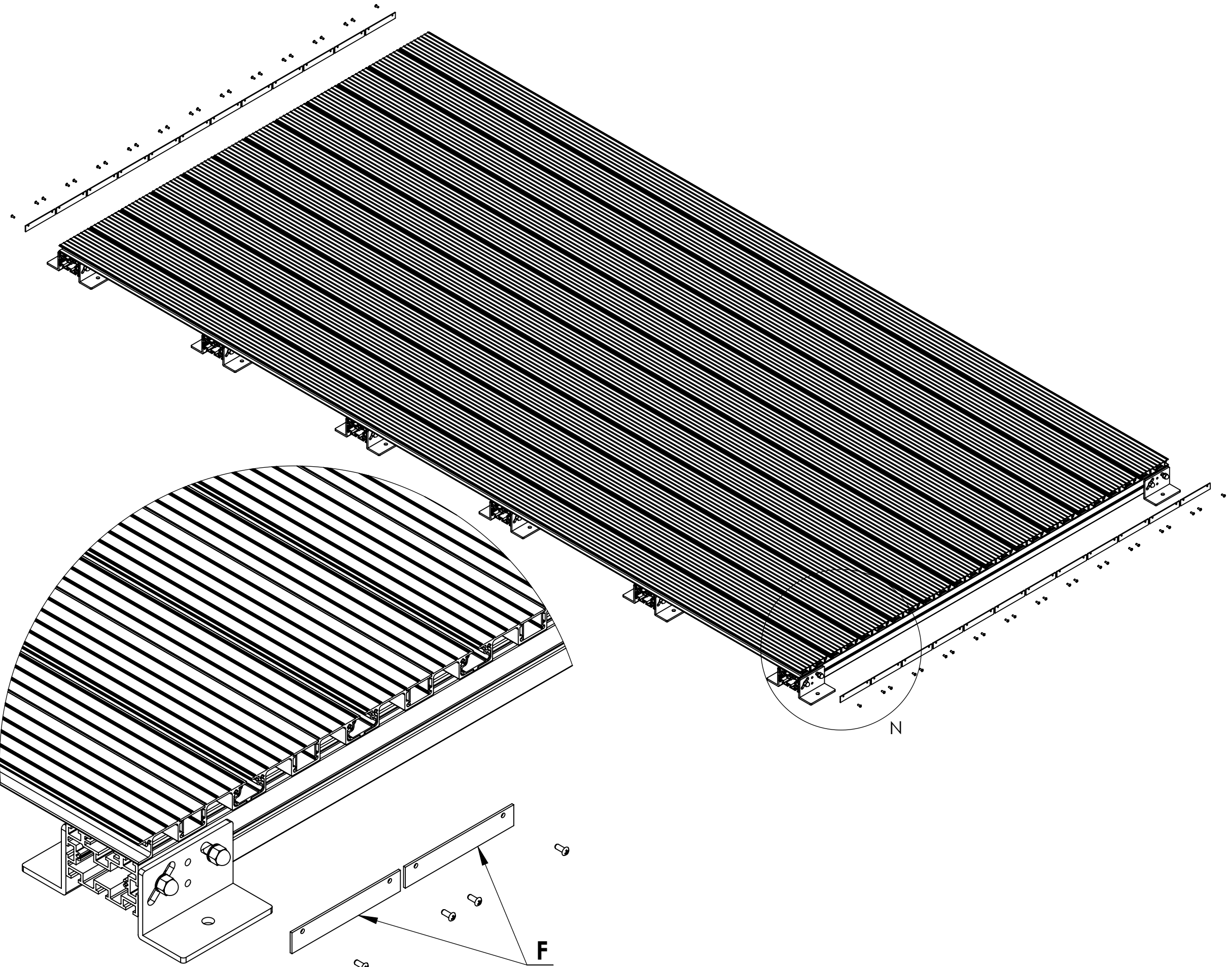
DETAIL N
