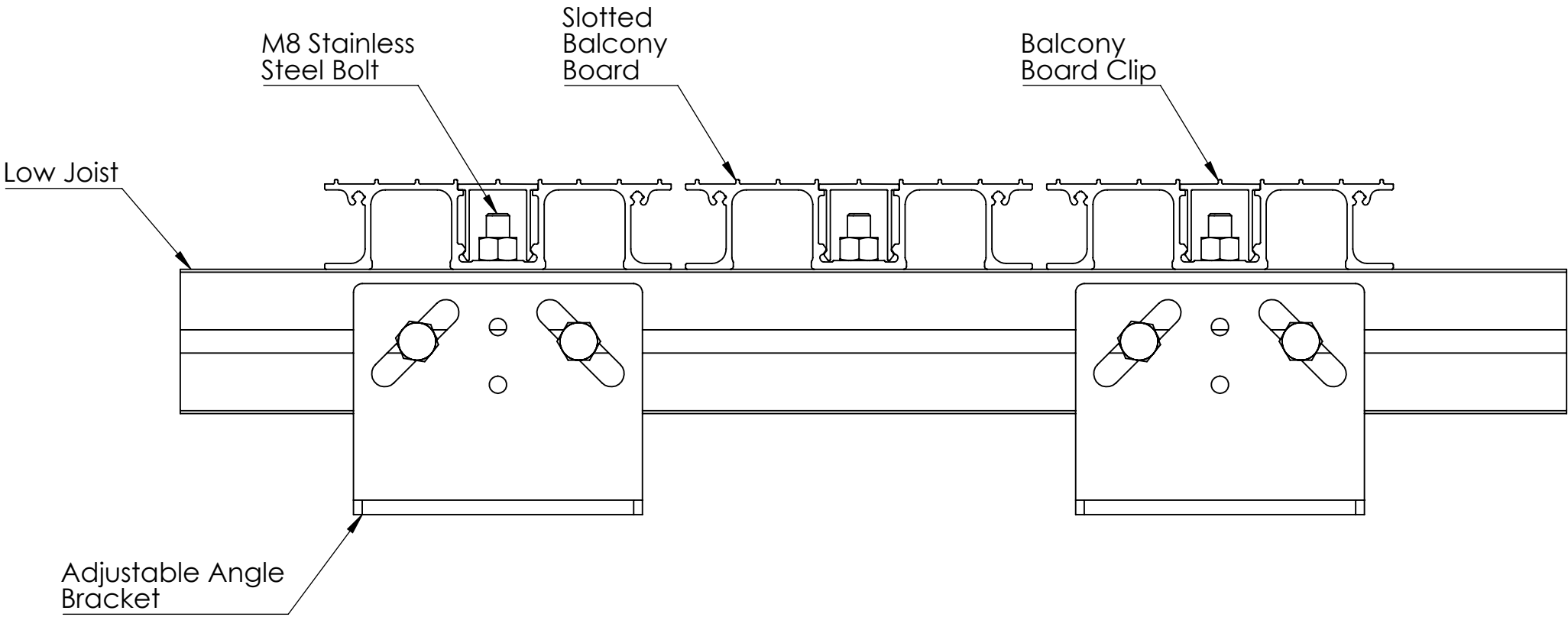
CROSS SECTION VIEW
