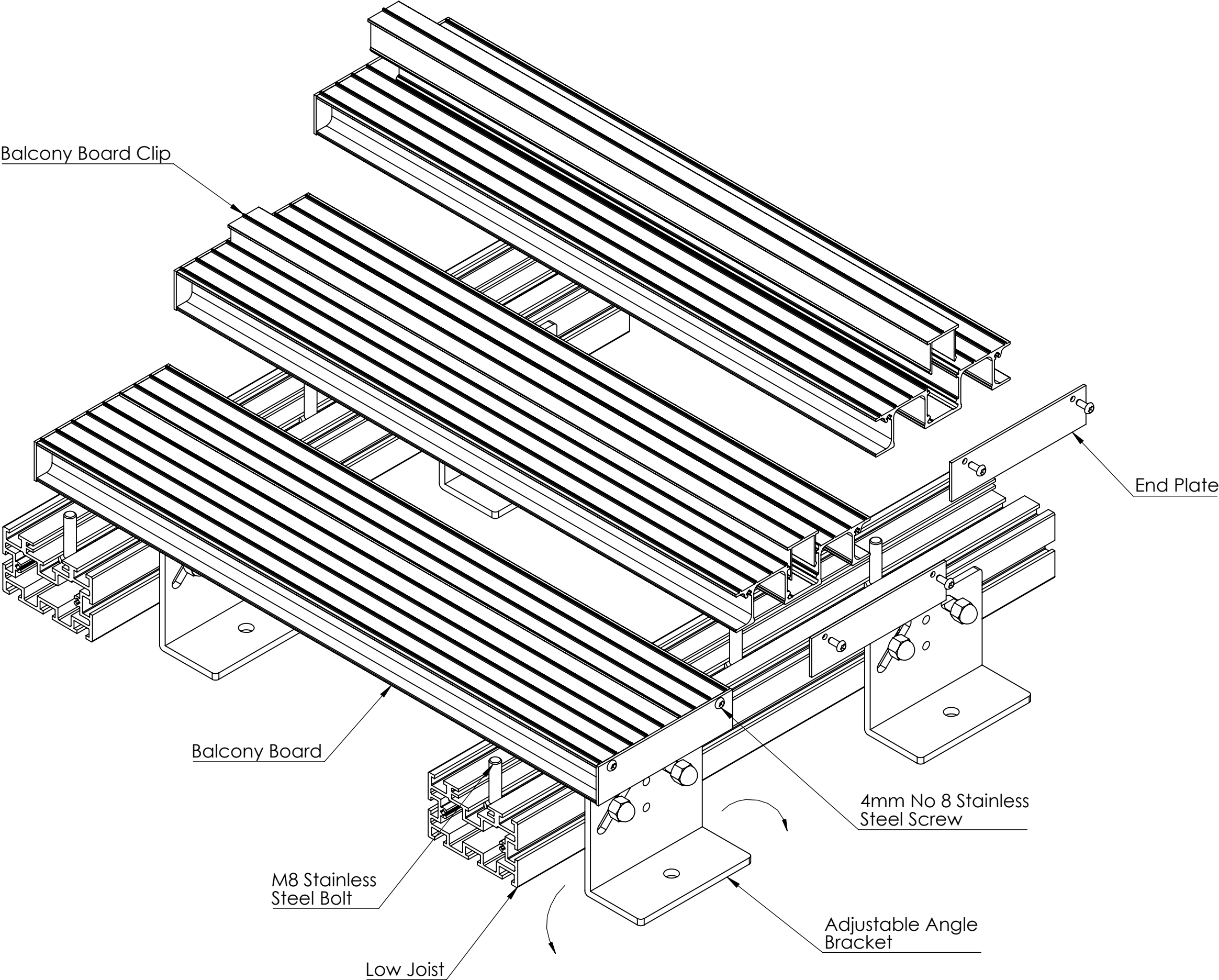
ISOMETRIC VIEW
