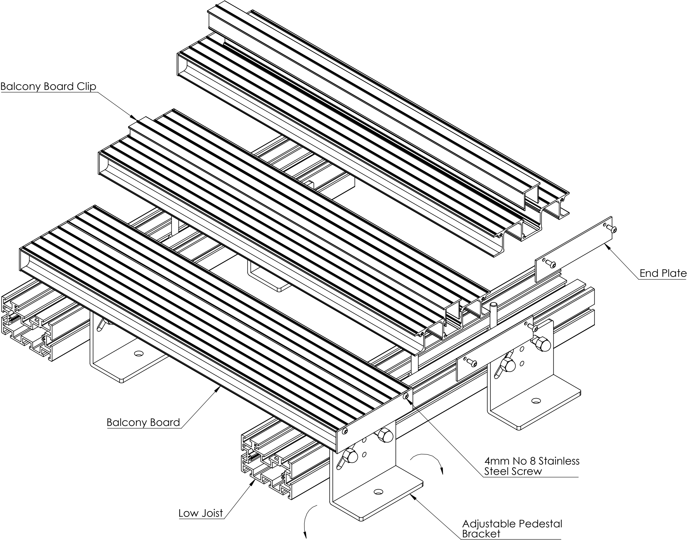
ISOMETRIC VIEW
